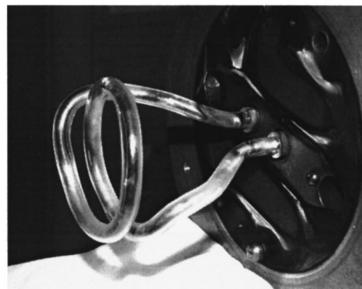
FIG. 5. Titanium tube antenna after 330 h of 2 kW cw operation in hydrogen plasma.
