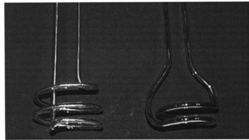
FIG. 4. On the left-hand side quartz antenna with the wire inside, on the right-hand side quartz antenna with the titanium tube inside.
